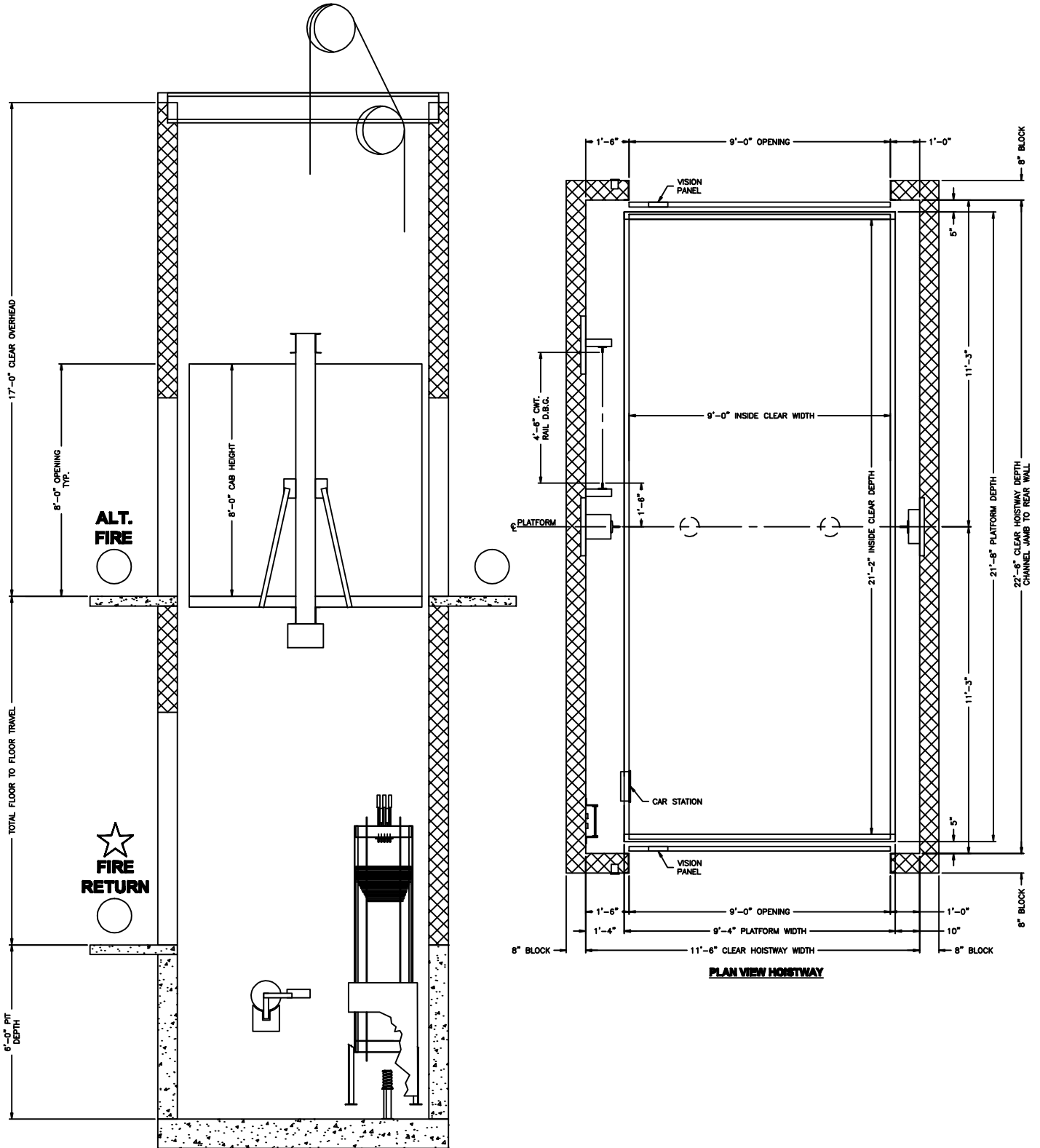
8000# CAPACITY F/R AUTOLIFT
