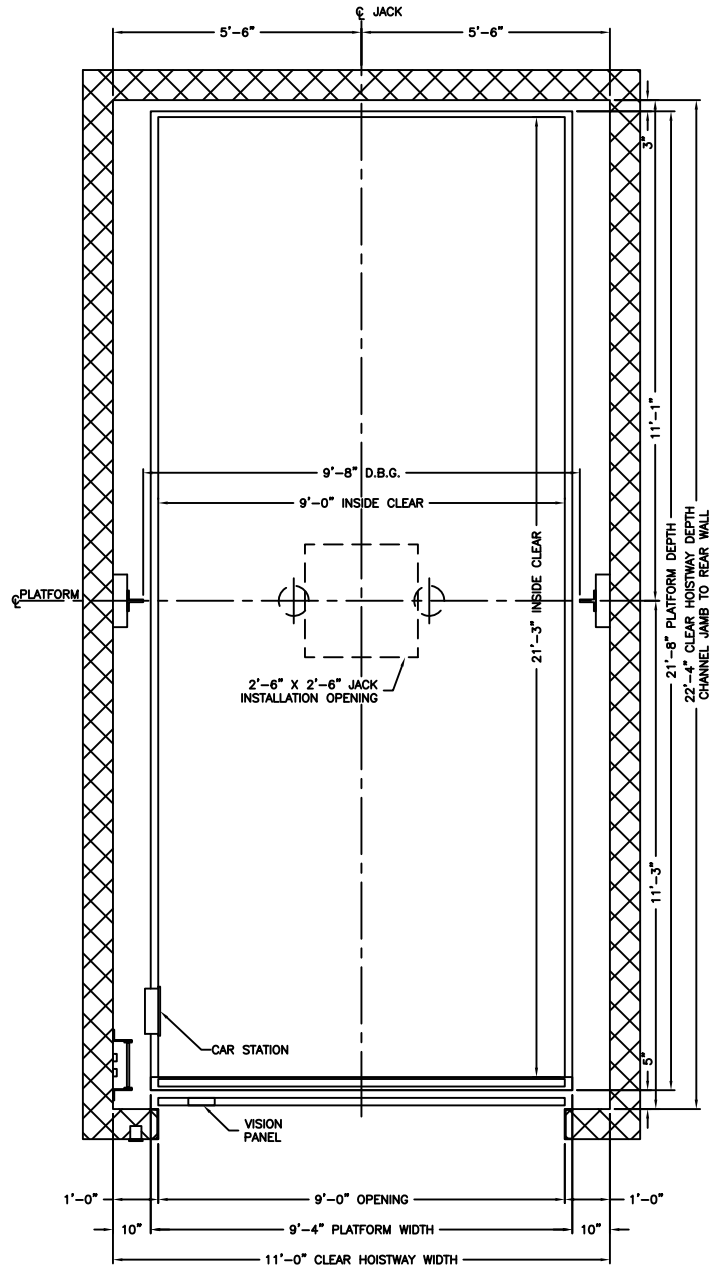
PLAN VIEW HOISTWAY
