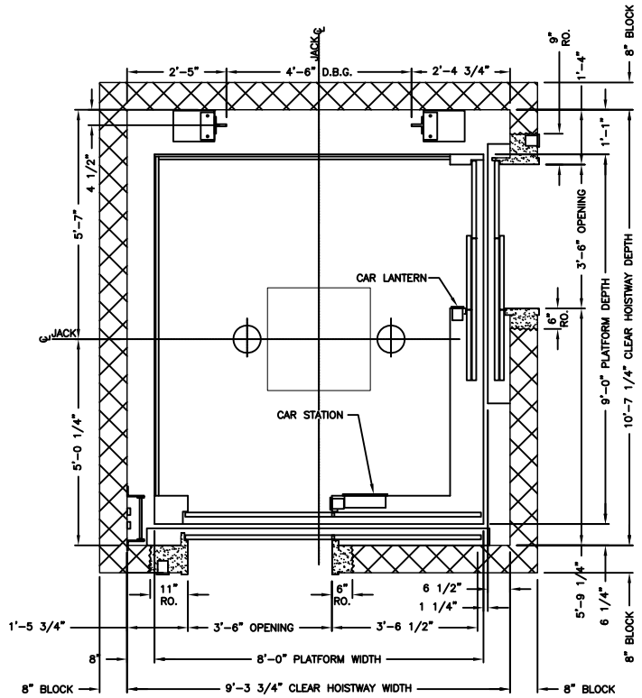
PLAN VIEW HOISTWAY
