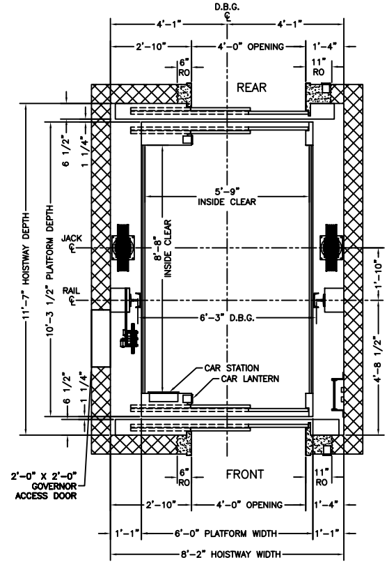
PLAN VIEW HOISTWAY
