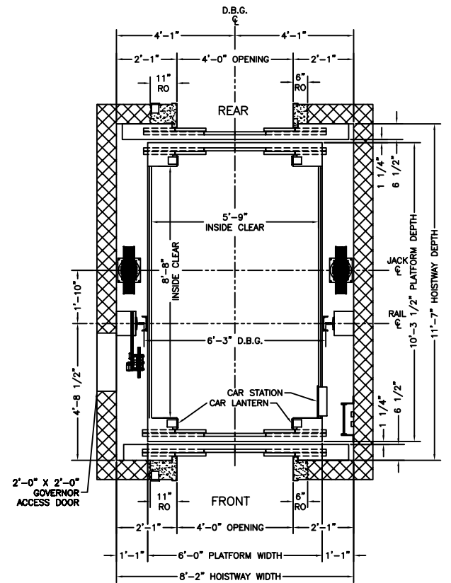
PLAN VIEW HOISTWAY
