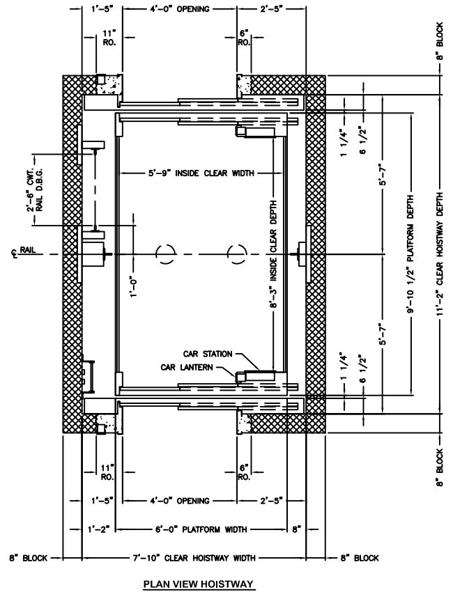
PLAN VIEW HOISTWAY
