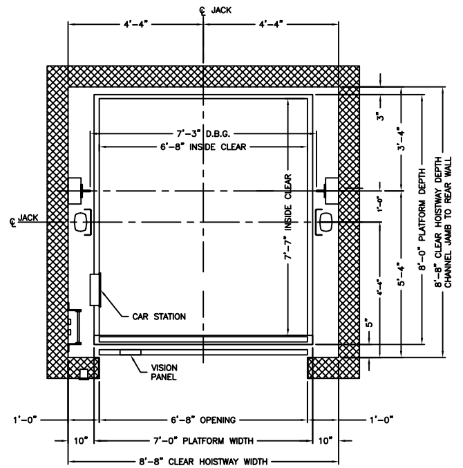
PLAN VIEW HOISTWAY
