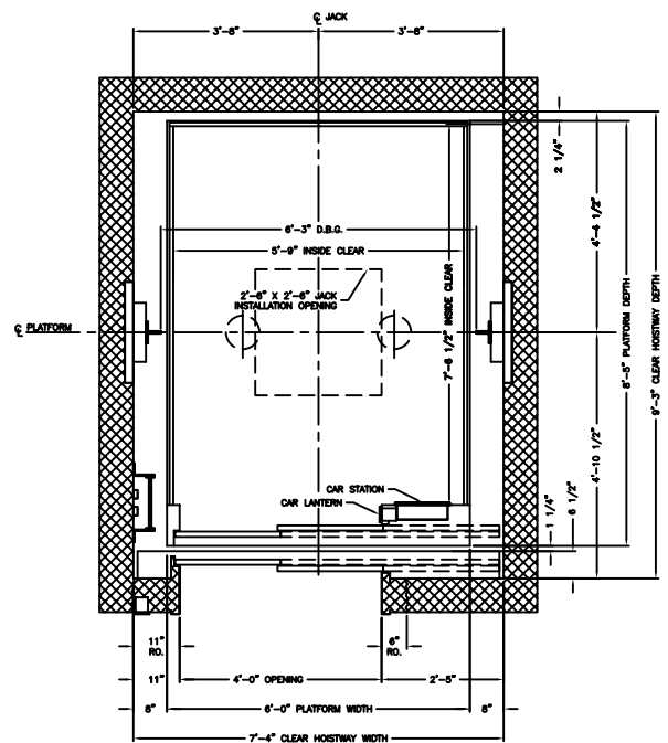
PLAN VIEW HOISTWAY
