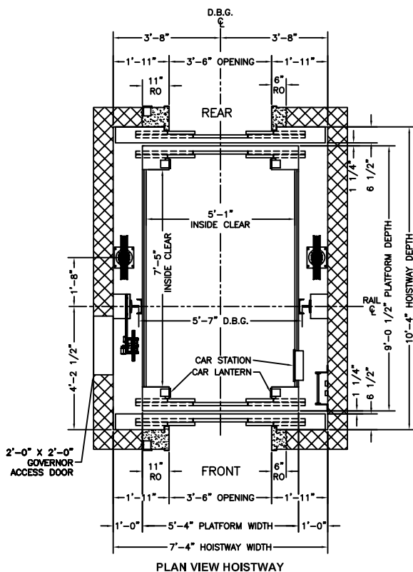
PLAN VIEW HOISTWAY
