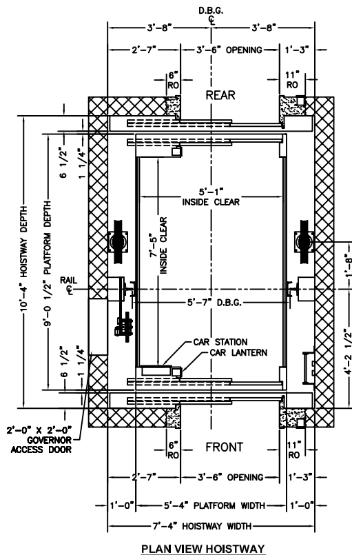
PLAN VIEW HOISTWAY
