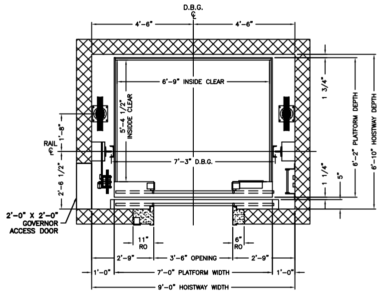
PLAN VIEW HOISTWAY
