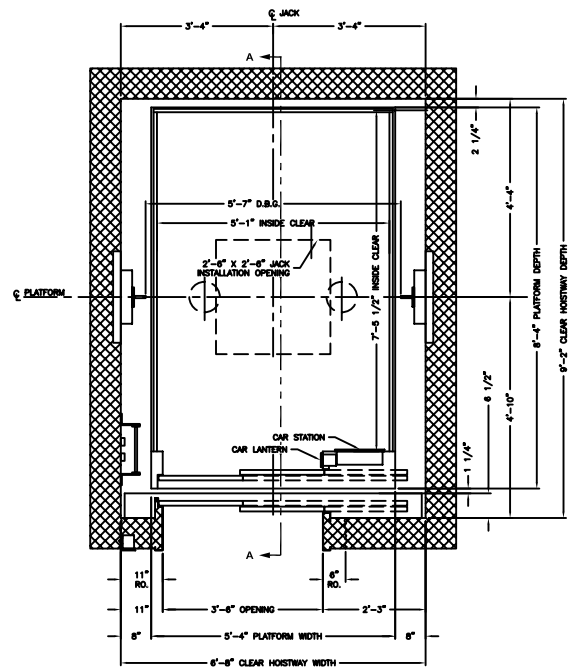
PLAN VIEW HOISTWAY
