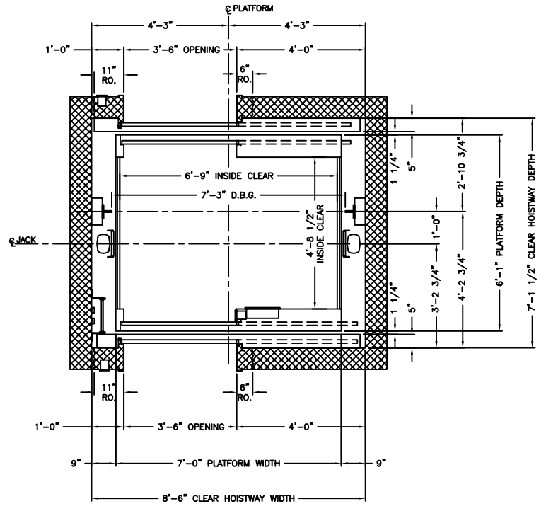
PLAN VIEW HOISTWAY
