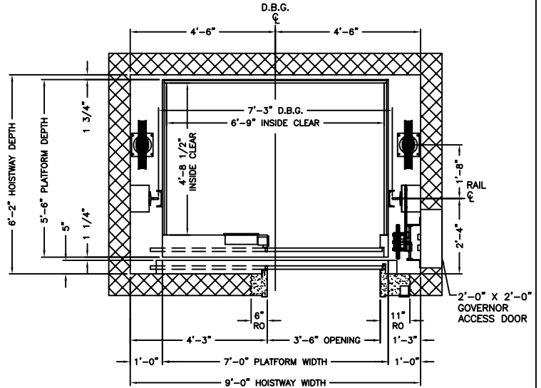
PLAN VIEW HOISTWAY
