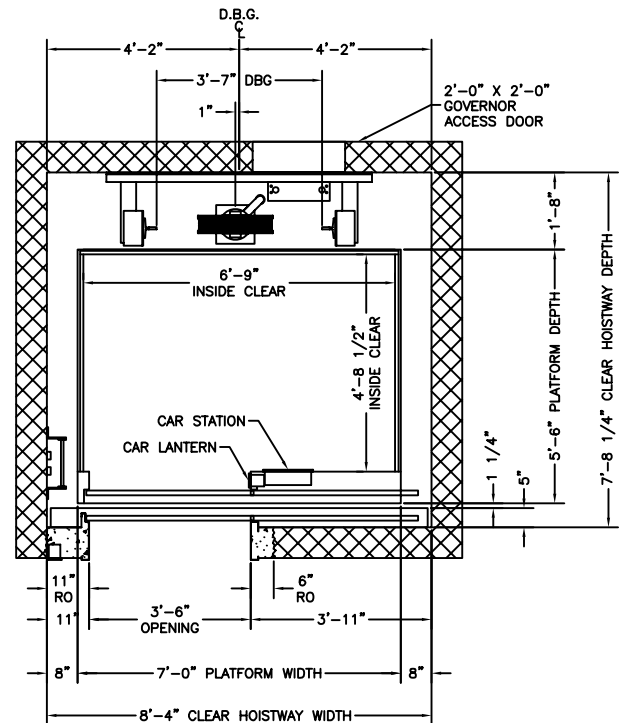
PLAN VIEW HOISTWAY
