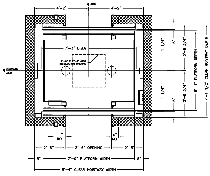
CENTER OPENING PLANVIEW
