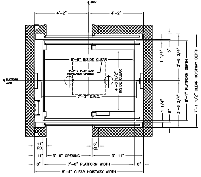
SIDE OPENING PLANVIEW
