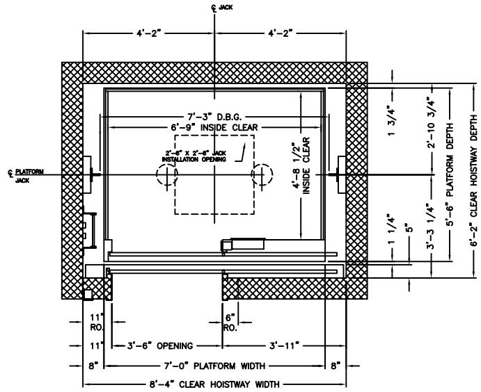
SIDE OPENING PLANVIEW
