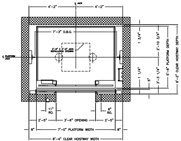
CENTER OPENING PLANVIEW
