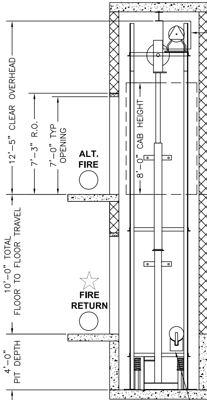
SECTION A-A ELEVATION VIEW
