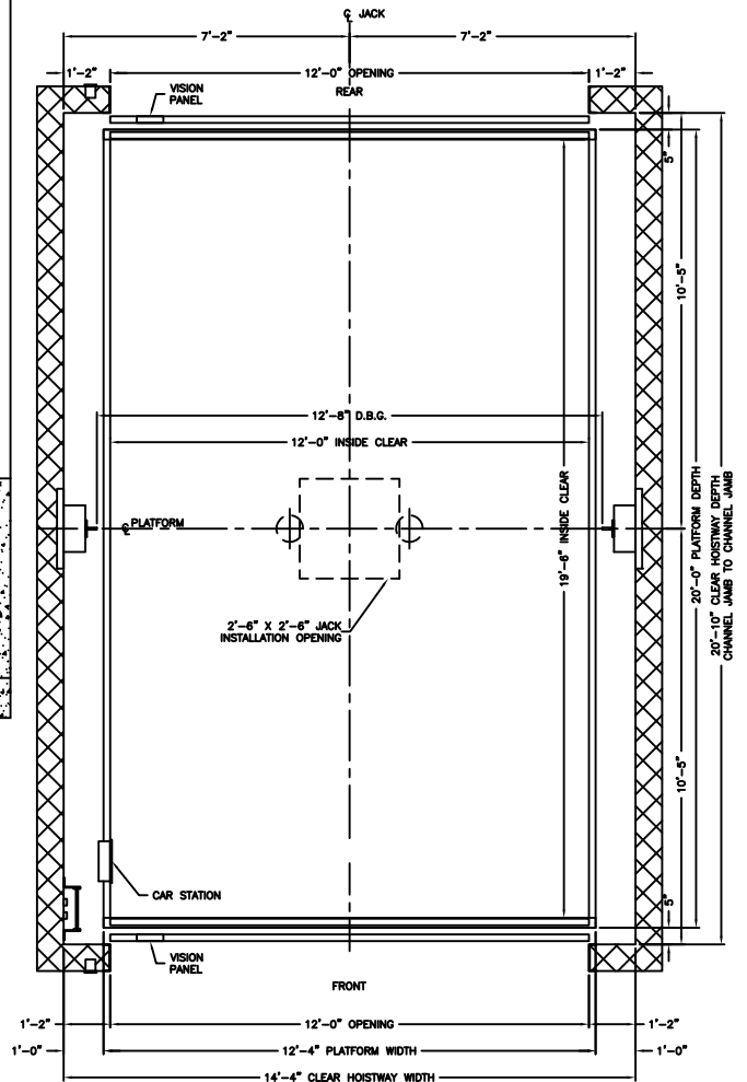
PLAN VIEW HOISTWAY
