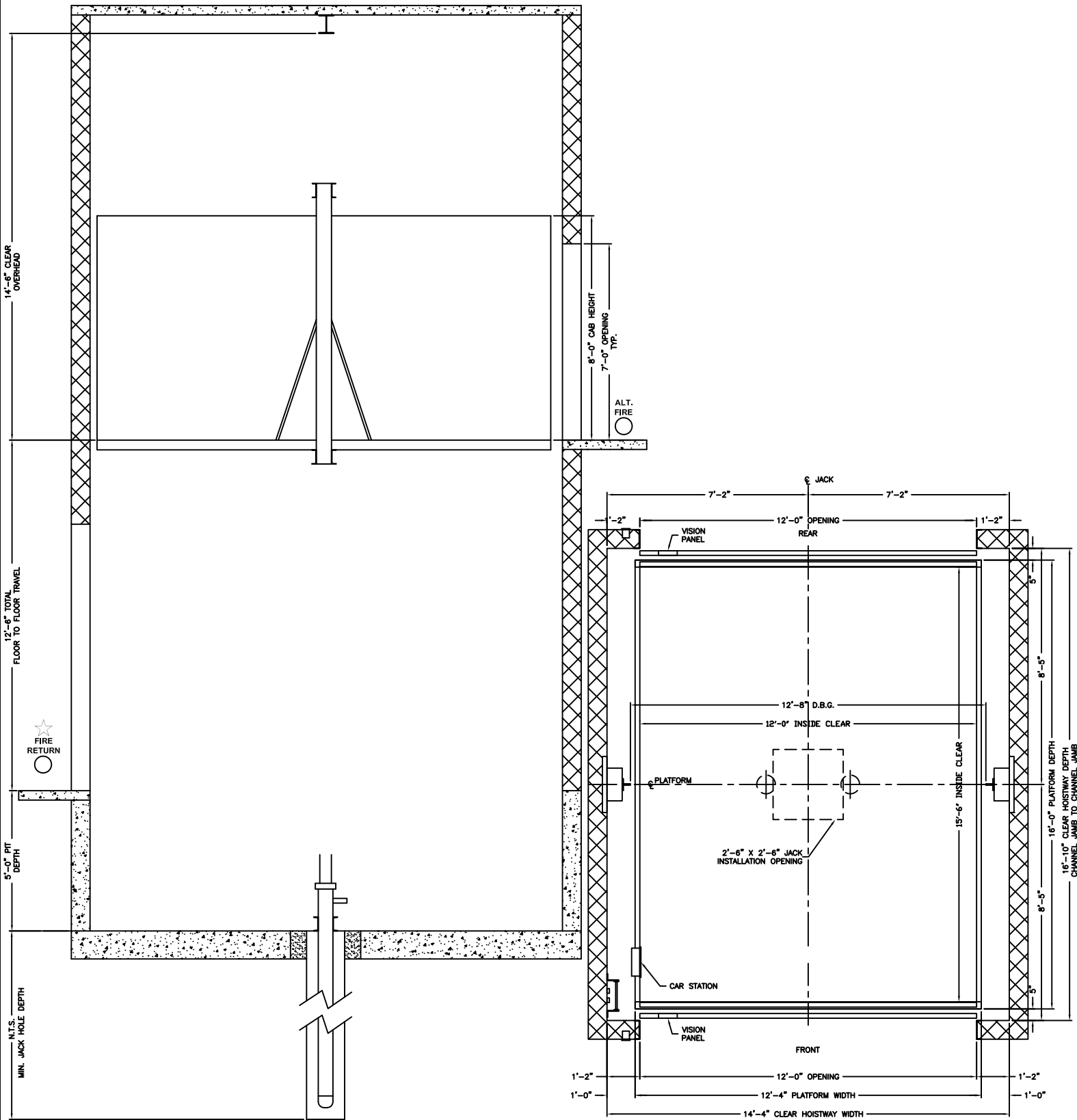
PLAN VIEW HOISTWAY
