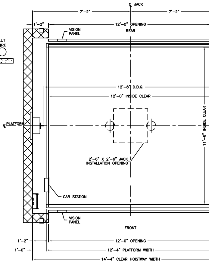
PLAN VIEW HOISTWAY
