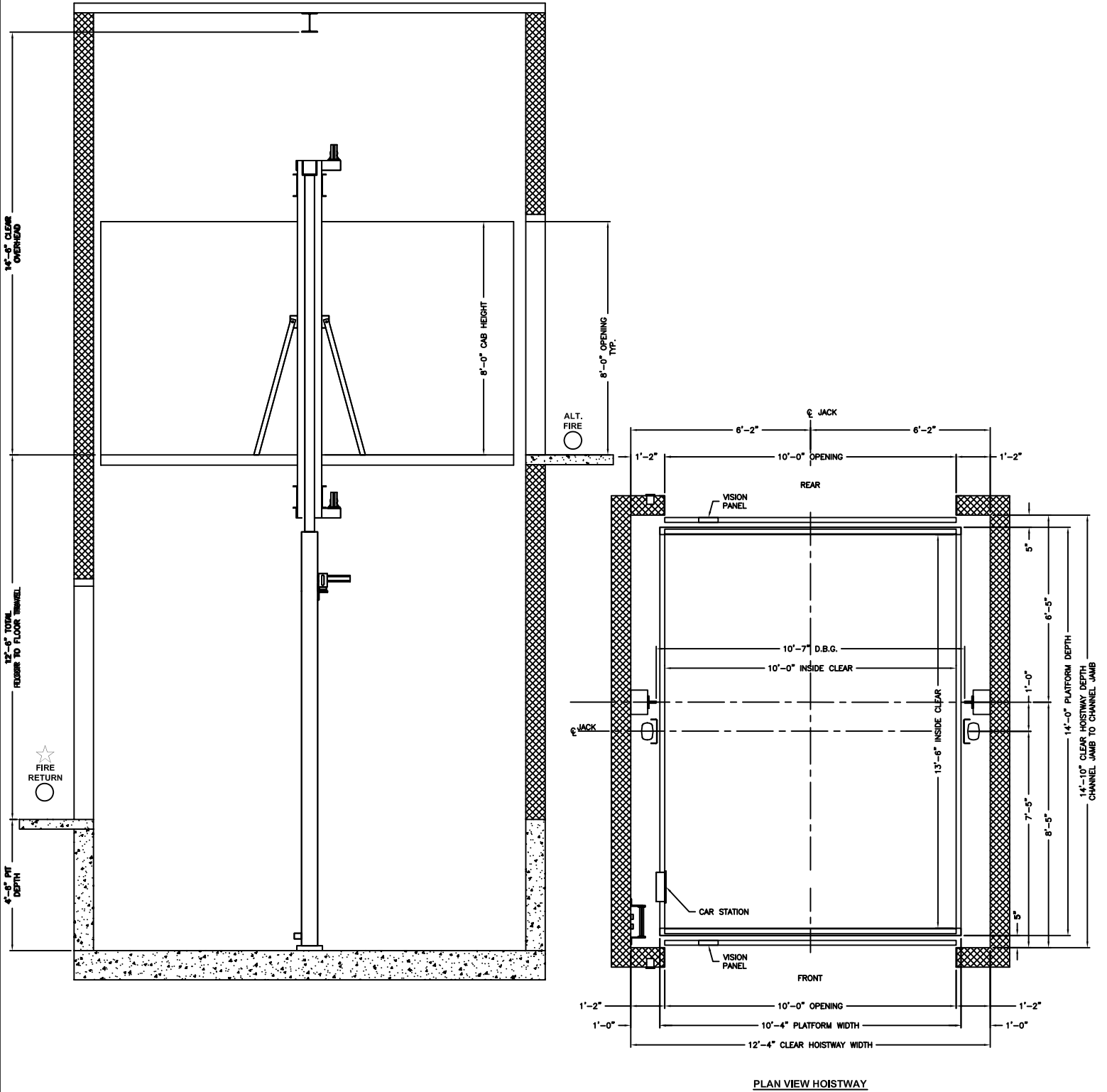
PLAN VIEW HOISTWAY
