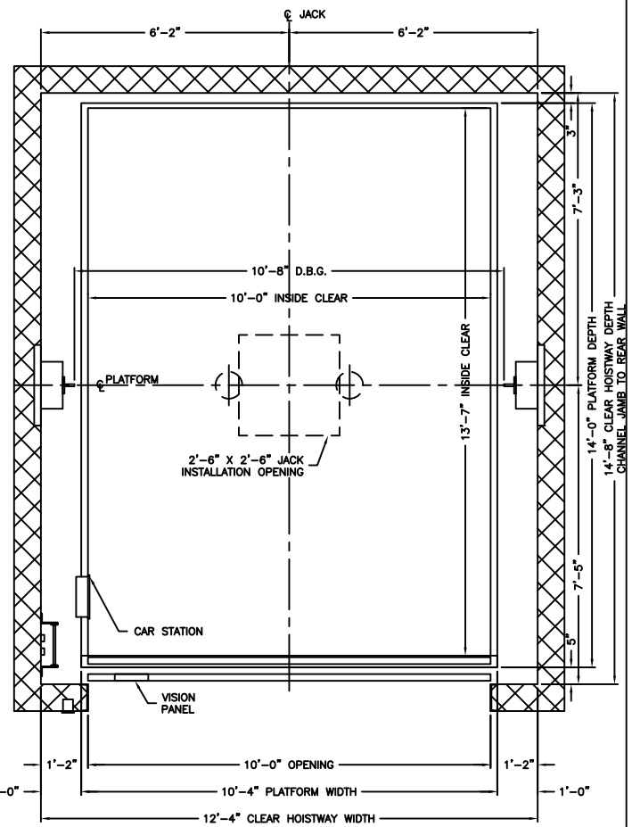
PLAN VIEW HOISTWAY
